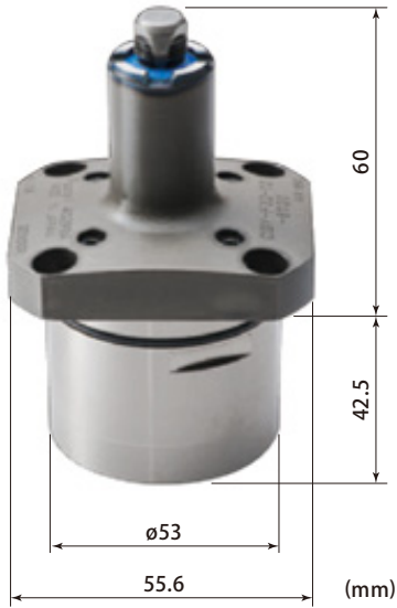
Expansion clamp CGY-F3
