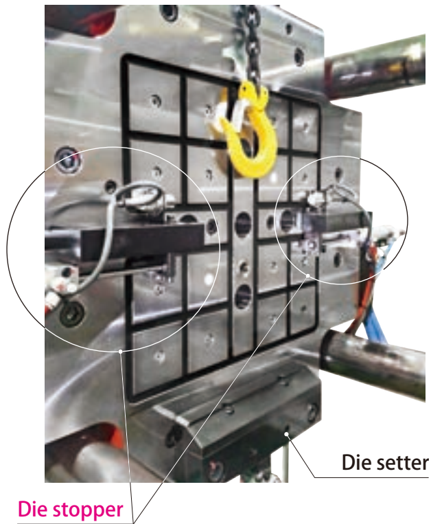
Movable platen
