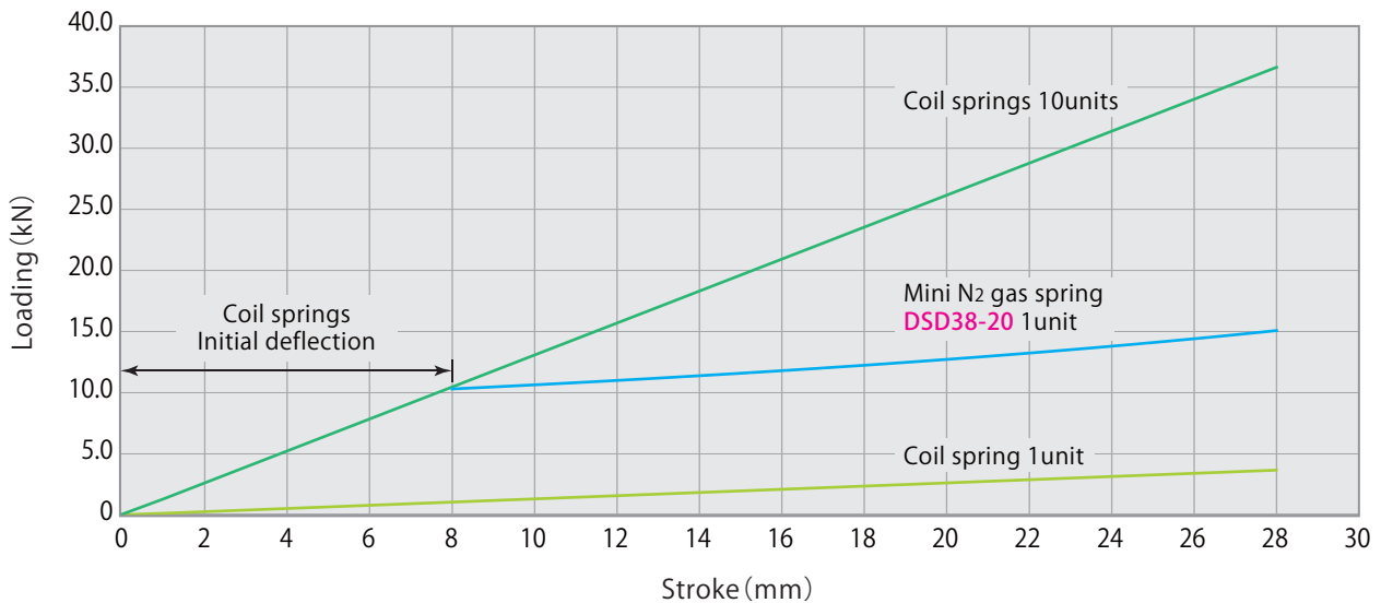
Load comparison between model DSD and coil spring
