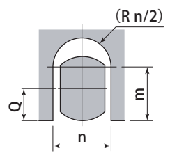
U-cut dimension
