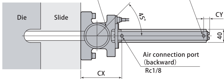
VIEW : X
