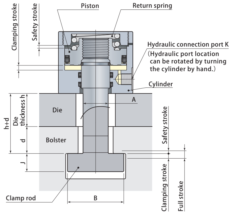
U-cut dimension
