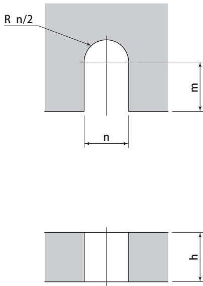
U-cut dimension
