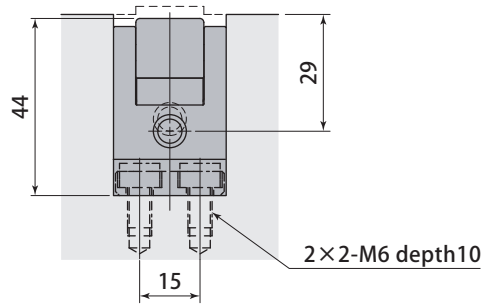
VIEW : Z
