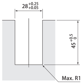
Slot details
