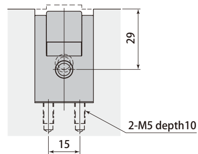
VIEW : Z
