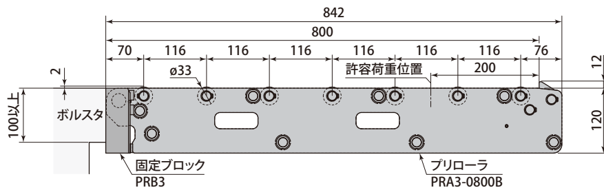
PRA3-0800B-S
