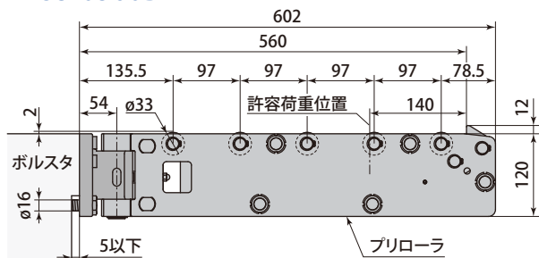
PRS3-0560B
