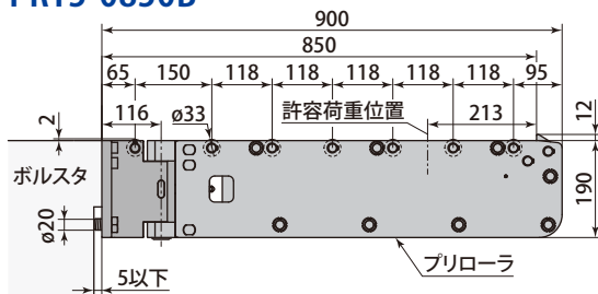
PRT5-0850B
