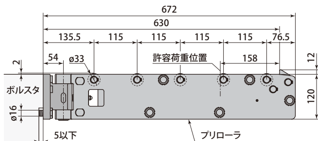
PRS3-0630B
