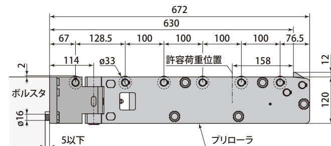
PRT3-0630B
