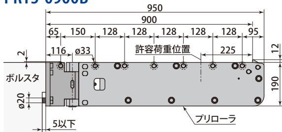
PRT5-0900B
