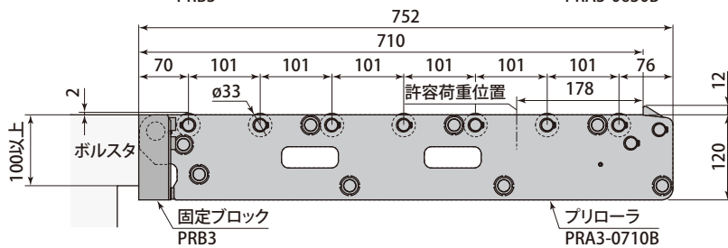
PRA3-0710B-S
