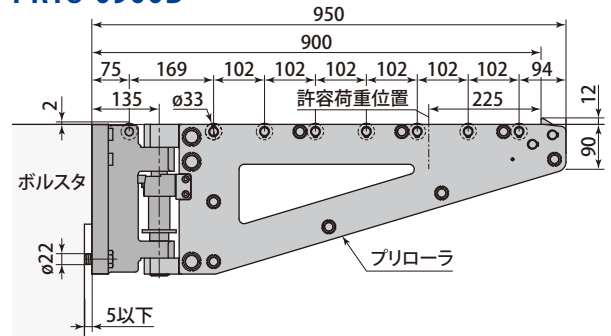
PRT8-0900B
