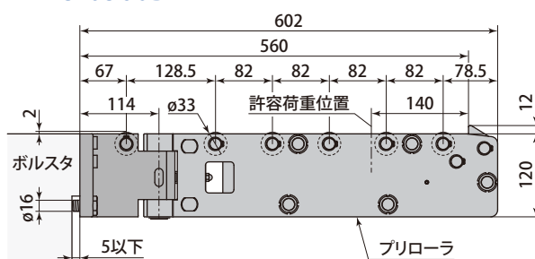
PRT3-0560B
