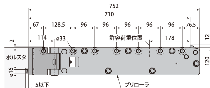
PRT3-0710B
