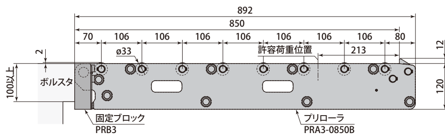
PRA3-0850B-S
