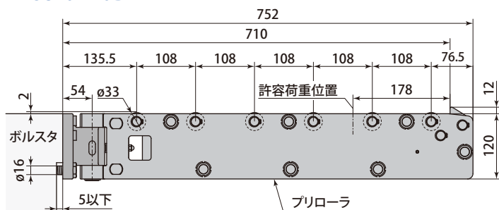
PRS3-0710B
